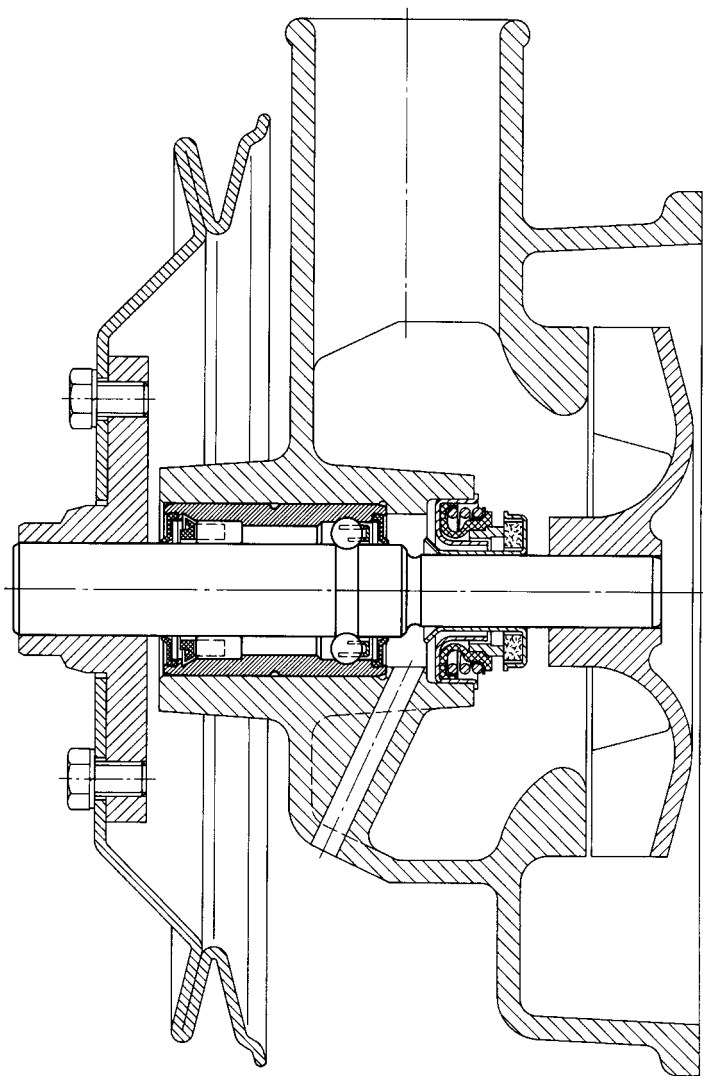
40: Water pump bearing unit for a truck engine
