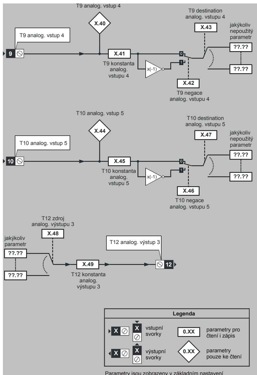
Obr. 10-26: I/O module analog logic diagram
