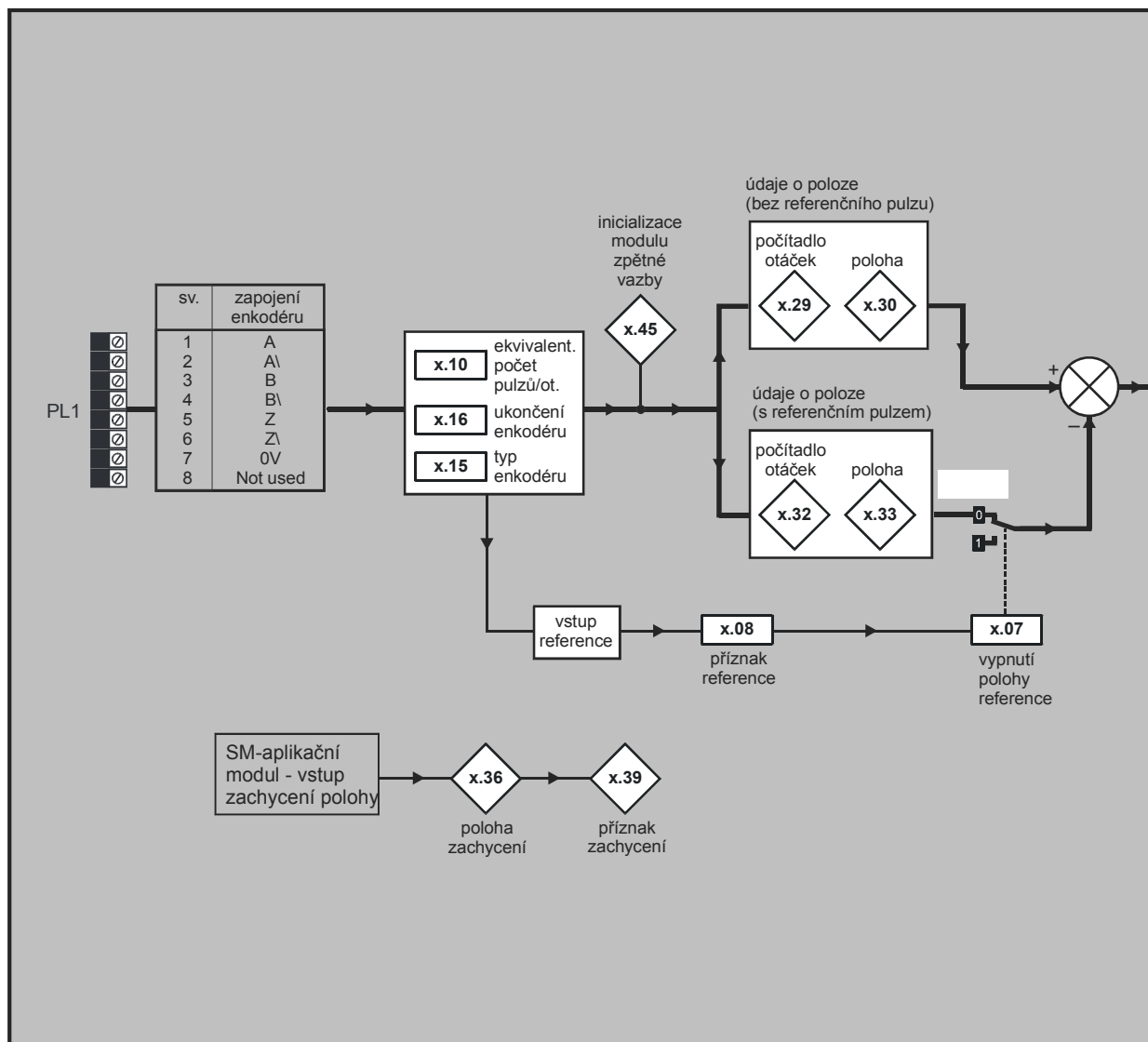
Obr. 10-25: SM-Encoder Plus logic diagram
