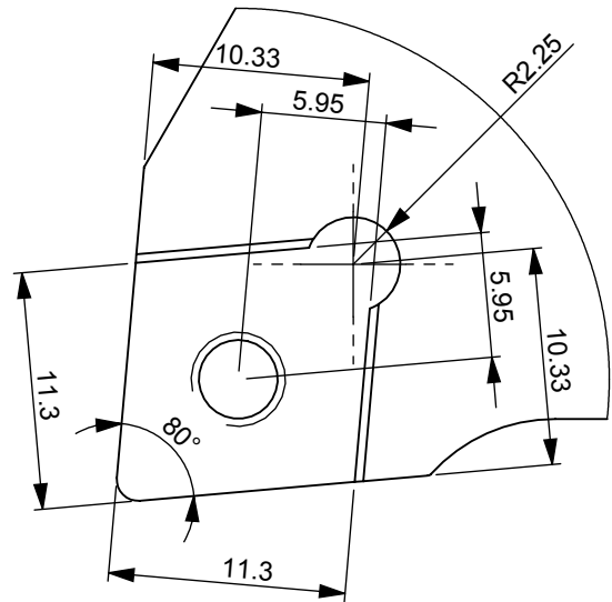
DETAIL D SCALE 5 : 2
