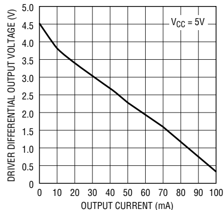
Driver Differential Output Voltage vs Output Current
