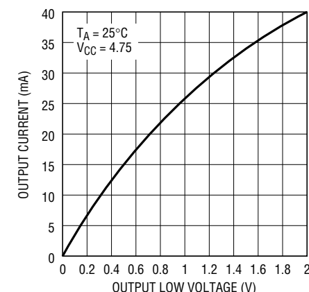
Receiver and Carrier Detect Output Low Voltage vs Output Current
