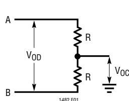
Figure 1. Driver DC Test Load #1
